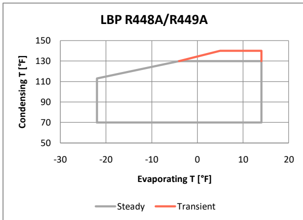
Fig.2 Restricted LBP R448A/R449A Envelope (max. superheat 18R)
