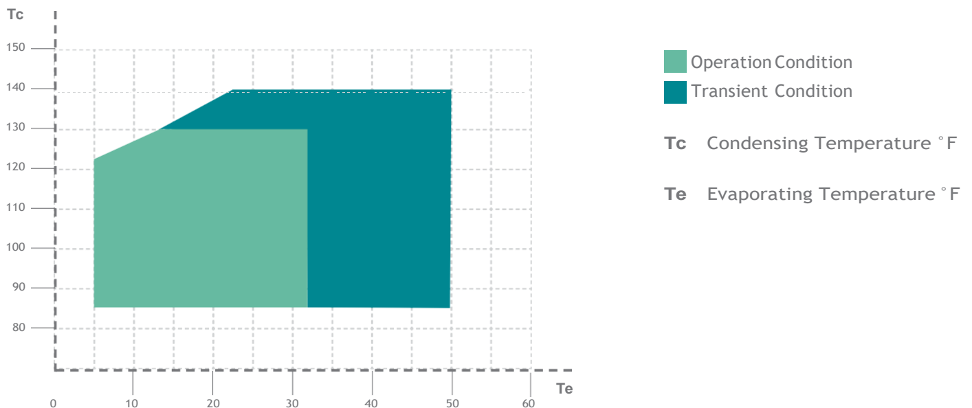
Fig.1 Restricted MBP R448A/R449A Envelope (max. return 68°F)
